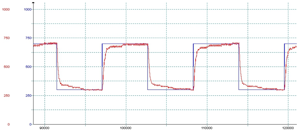
Fig. 14: Test scenario with the control parameters P = 100,000 , I = 5,000 , D = 400
