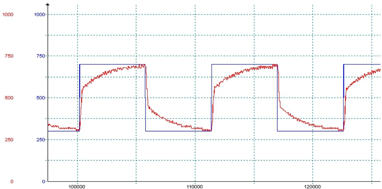
Fig. 13: Test scenario with the control parameters P = 100,000 , I = 5,000 , D = 0
