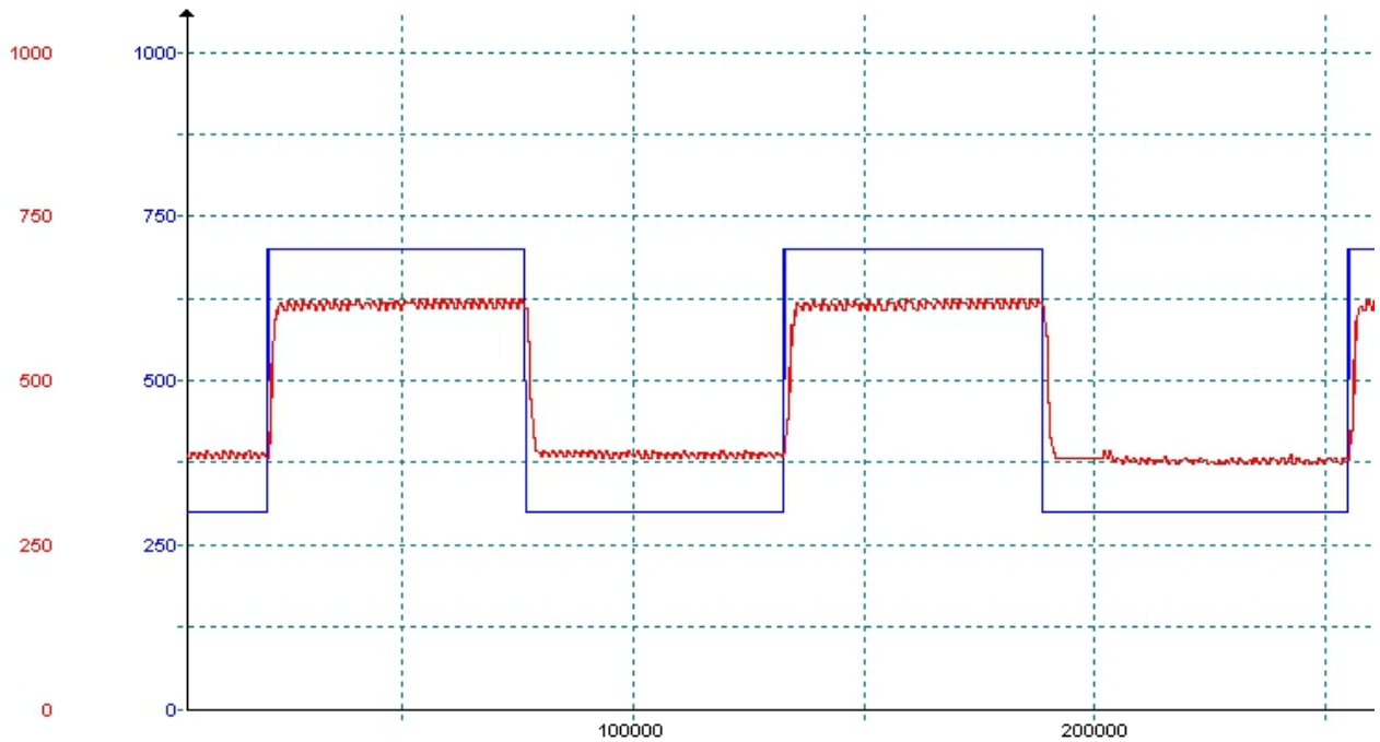
Fig. 12: Test scenario with the control parameters P = 100,000 , I = 0 , D = 0
