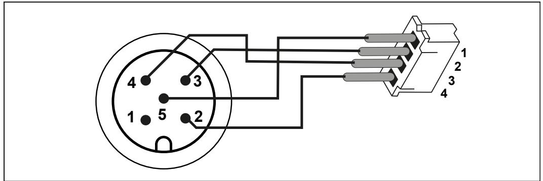
Fig. 9: M12 plug, 5-pin, A-coded
