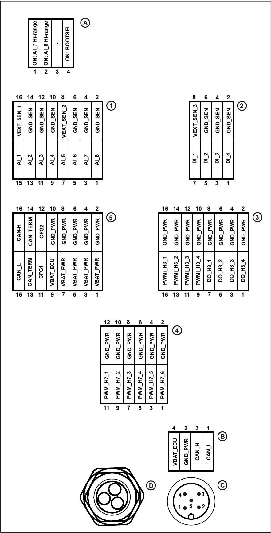
Fig. 7: PCB - pin assignment (top view)
