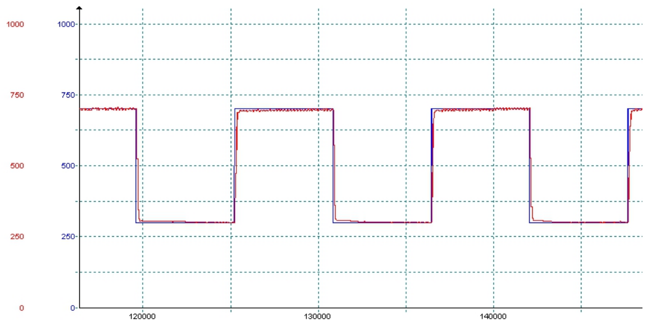
Fig. 15: Test scenario with the control parameters P = 100,000 , I = 10,000 , D = 400
