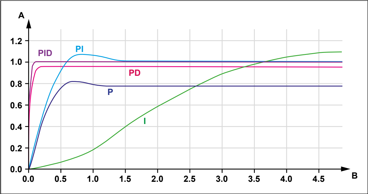
Fig. 11: Comparison of controller types in a control loop
